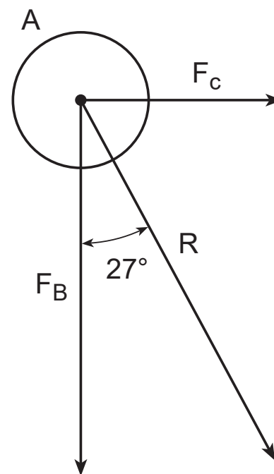
Gravitational Force on Mass A
