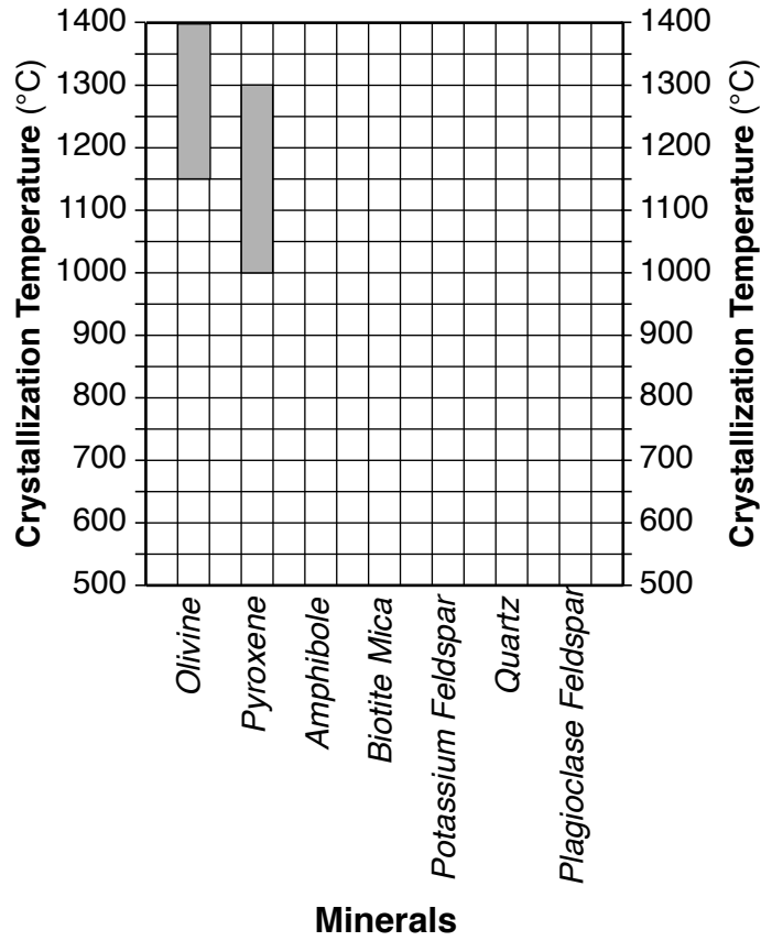
Crystallization Temperatures of Minerals Commonly Found in Igneous Rocks
